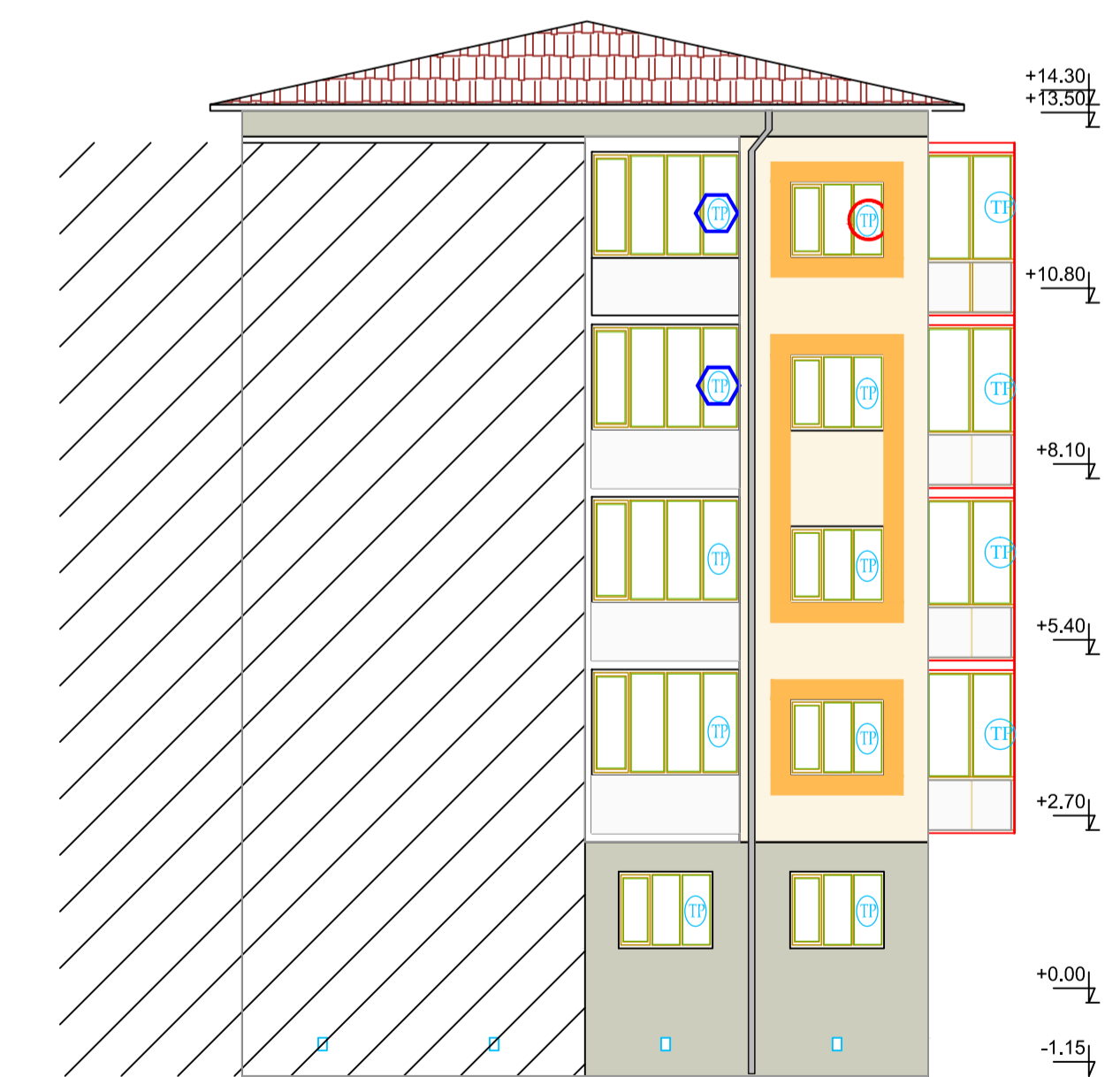
FATADA LATERALA STANGA PROPUSA
